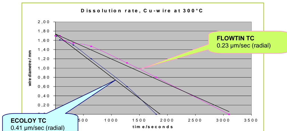
Radial dissolution of copper wire in FLOWTIN® TC solder bath @300°C
